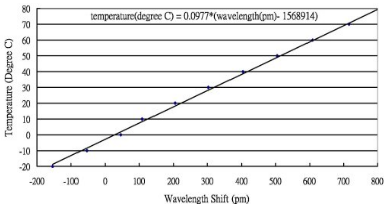
FBG Temperature Sensor Calibration Curve
